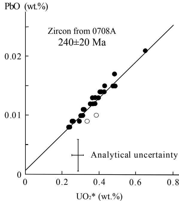
Fig. 5. Plots of PbO vs. \text{UO}_2^* for zircon grains from adamellite sample 0708A in the Hirasawa Mass. Open circles represent rim of euhedral grain Z10. Explanation for errors is the same as for Fig. 4.
