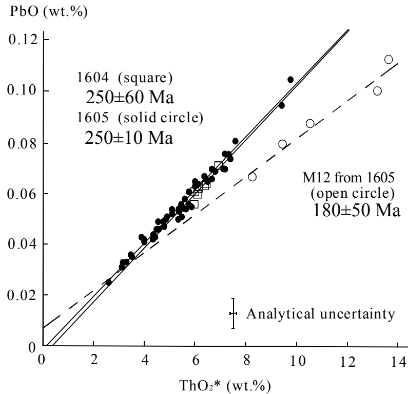
Fig. 6. Plots of PbO vs. ThO 2 * for monazite from leucocratic adamellite (sample Nos. 1604 and 1605) collected at the mouth of the Kusayami-zawa. Analytical data are given in Appendix 2. Explanation for errors is the same as for Fig. 4.
