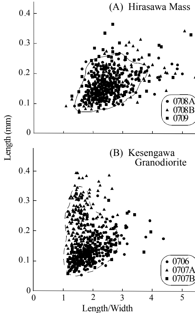
Fig. 3. Plots of length vs. elongation (length/width) for zircon grains from three adamellite samples (sample Nos. 0708A, 0708B and 0709) in the Hirasawa Mass (A) and two granodiorite samples (sample Nos. 0706 and 0707A) and a leucocratic granite sample (sample No. 0707B) in the Cretaceous Kesangawa Granodiorite (B). Solid and dashed lines in the figures represent 1 % contour of distribution intensity defined in an area of 0.4X0.04 scale units.
