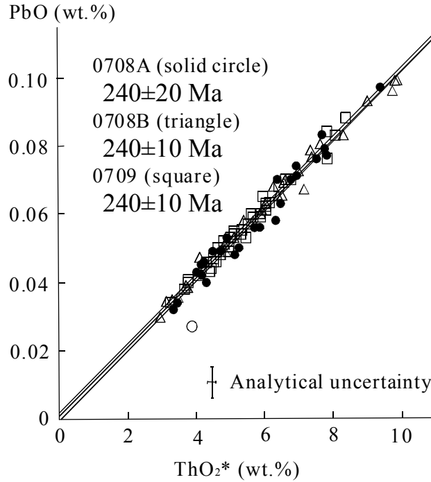
Fig. 4. Plots of PbO vs. ThO 2 * for monazite grains from three adamellite samples (sample nos. 0708A, 0708B and 0709) in the Hirasawa Mass. Open circle represents core of small grain M12 from sample 0708A. Error bars in the figure represent 2\sigma analytical uncertainty, and errors given to the age are of 2\sigma .
