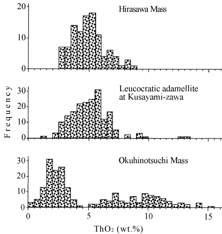
Fig. 8. Frequency distribution diagram of \text{ThO}_2 in monazite grains from adamellite in the Hirasawa Mass, leucocratic adamellite at Kusayami-zawa and leucogranite in the Okuhinotsuchi Mass. Th-rich monazite grains from leucogranite in the Okuhinotsuchi Mass, giving ca. 430 Ma CHIME age (Adachi et al., in press), are xenocrysts.
