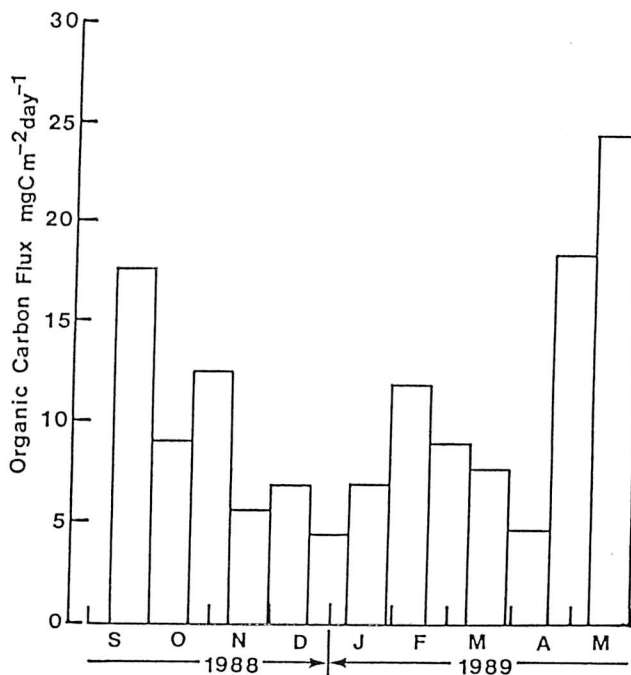
Fig. 4 Vertical flux of organic carbon in the Japan Trench
