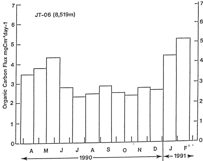
Fig. 2 Vertical flux of organic carbon in the Izu-Ogasawara Trench
