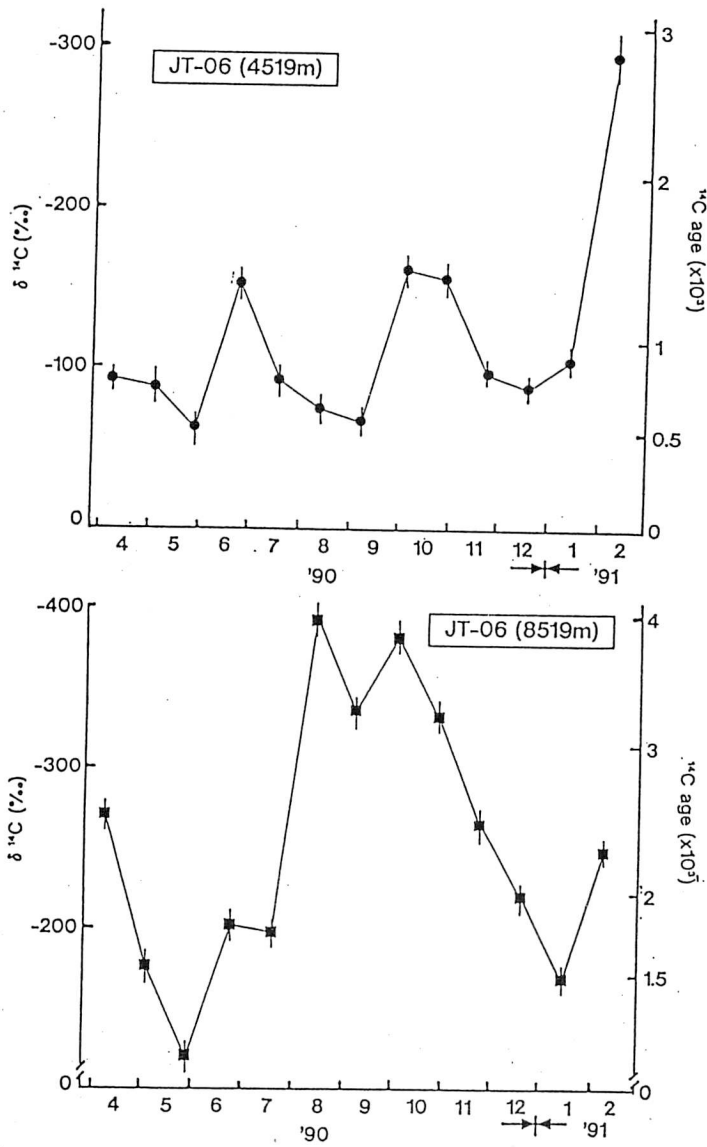
Fig. 3 Change in \delta^{13}C of the sinking particles from Izu-Ogasawara
