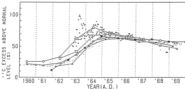
Fig.8 \delta^{14}\text{C} values in a Hinoki (35.6°N,137.5°E Nakamura et al.,1987)( \diamond ), a Merkusii Pine(11°N, 107°E)( \square ), a Teak(7°S, 111°E)( \triangle ), a Araucaria(27°S, 50°W)( \blacksquare ), and a Lingue (38°4'S,71°54'W)( \blacktriangle ) compared with atmospheric \Delta^{14}\text{C} values measured in Northern Spain (42°53'N, 8°26'W)( \circ ), Ethiopia(8°40'N, 38°58'E)( \square ), and Madagascar(21°27'S, 47°5'E)( \triangle ) (Nydal et al., 1983), Fiji(18°S, 178°W)( \diamond ) and New Zealand(41°18'S, 174°14'W)( \nabla ) (Rafter,1965).
