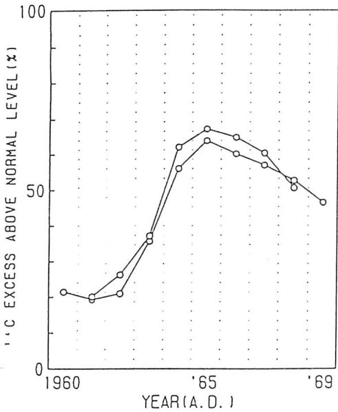
Fig.4 \delta^{13}\text{C} values in two Teaks cut down in the same forest.
