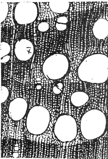
Photo.4 Cross section of a Teak. X40.
