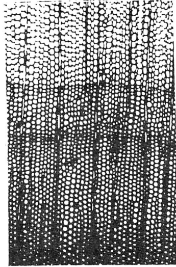
Photo. 3 Cross section of a Parana Pine.False annual ring. X30.
