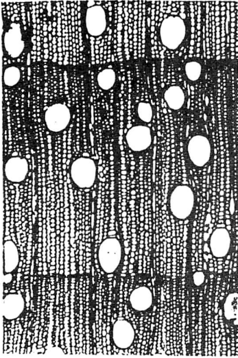
Photo.2 Cross section of a Lingue. X40.
