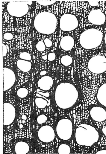
Photo.5 Cross section of a Teak. Narrow-ring. X40.
