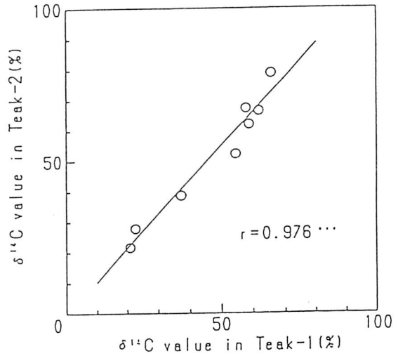
Fig.5 Relationships of \delta^{13}\text{C} values between two Teaks cut down in the same forest.
