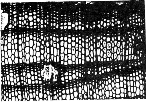
Photo.1 Cross section of a Merkusii Pine. False annual ring. X40.
