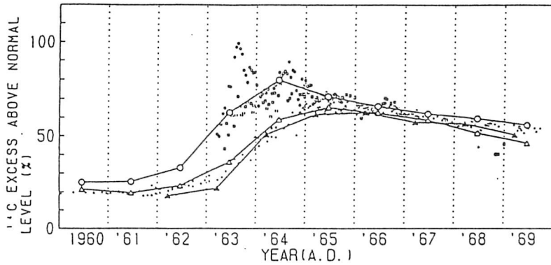
Fig.7 \delta^{14}\text{C} values in a Hinoki (35.6°N,137.5°E Nakamura et al.,1987)( \diamond ), a Teak(7°S, 111°E)( \square ), and a Lingue (38°4'S,71°54'W)( \triangle ) compared with atmospheric \Delta^{14}\text{C} values measured in Northern Spain(42°53'N, 8°26'W)( \circ ), Ethiopia(8°40'N, 38°58'E)( \square ), and Madagascar(21°27'S, 47°5'E)( \triangle )(Nydal et al., 1983), Fiji(18°S, 178°W)( \diamond ) and New Zealand(41°18'S, 174°14'W)( \nabla )(Rafter,1965).
