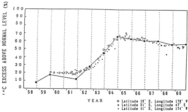
Fig.6 Carbon 14 variation in an Araucaria and in the troposphere at various latitudes
