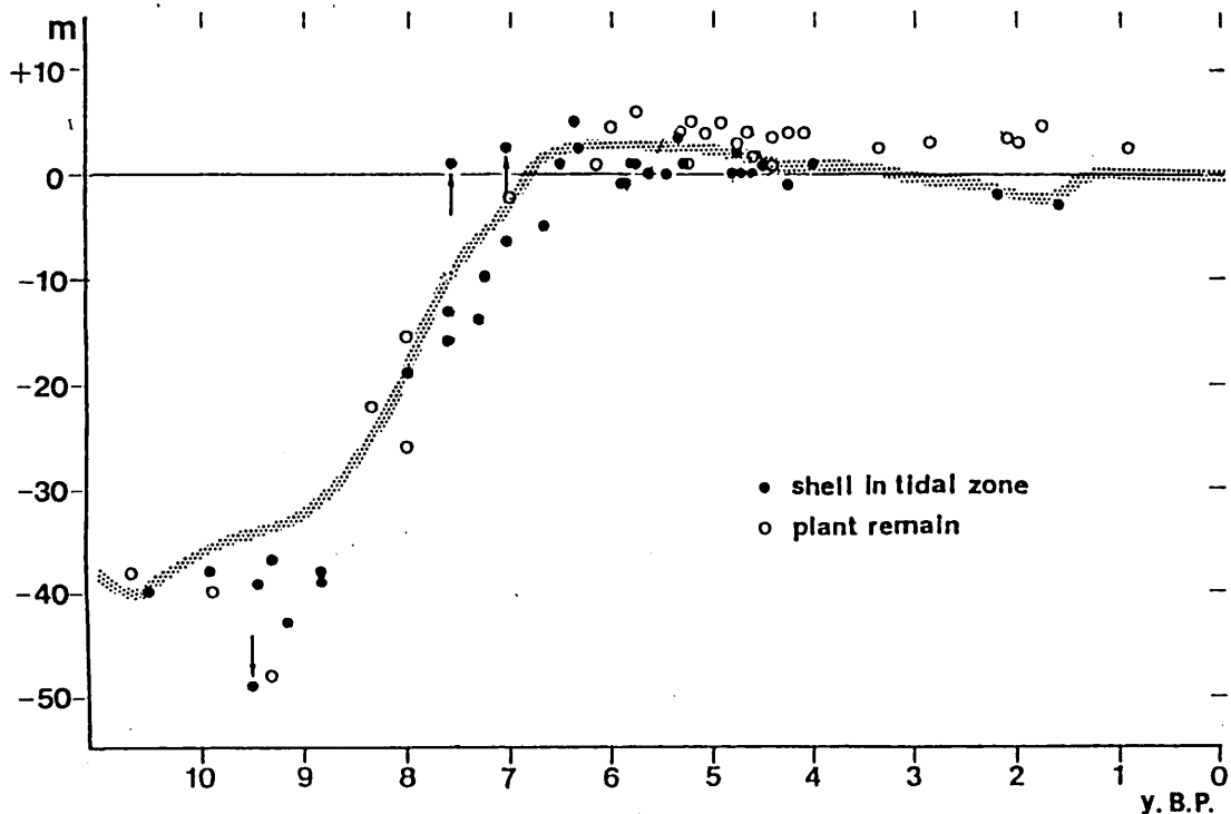
Fig. 1 Relative sea-level curve during the last 10,000 years from the Paleo-Okutokyo Bay and its surroundings. (Endo et al. 1989)
