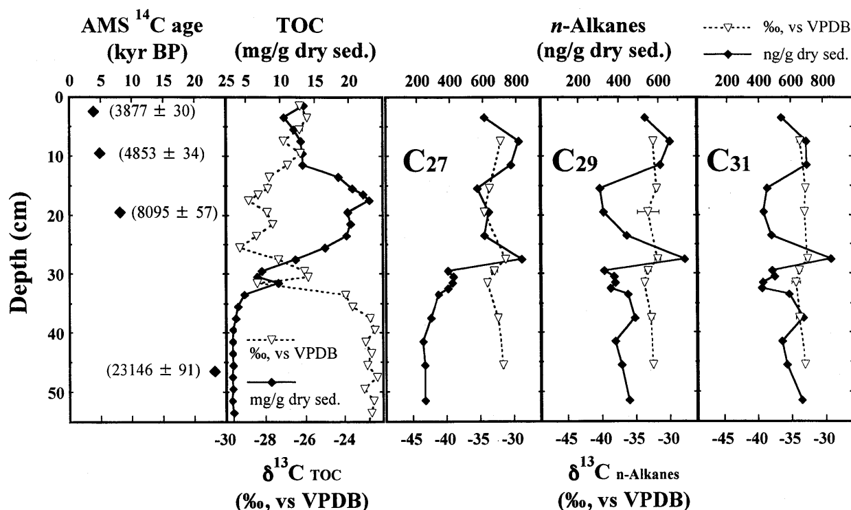
Figure 1. Depth profiles of AMS ^{14}\text{C} age as well as concentrations and stable carbon isotope ratios of total organic carbon (TOC) and n-alkanes (C 27 , C 29 and C 31 ) in the Ver98-1 St.5 sediment core.
