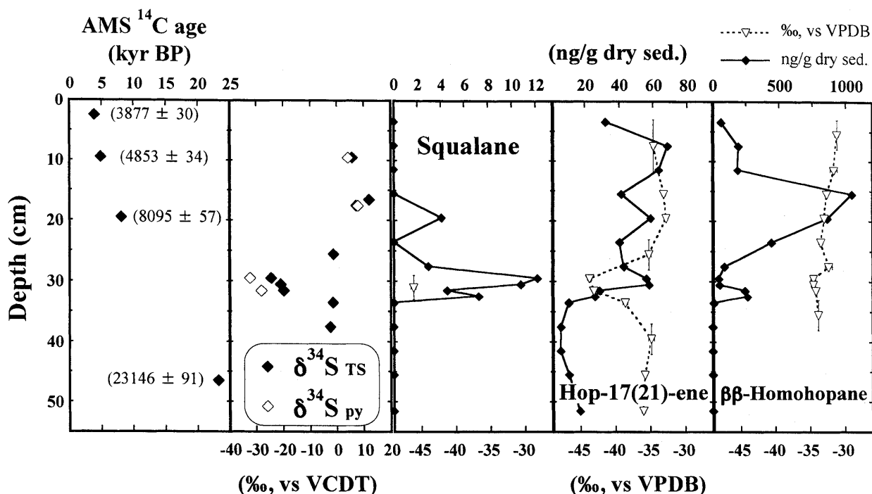
Figure 2. Depth profiles of AMS ^{14}\text{C} age, stable sulfur isotope ratios of total sulfur and pyrite ( \delta^{34}\text{S}_{\text{TS}} , \delta^{34}\text{S}_{\text{py}} ), concentrations and stable carbon isotope ratios of squalane, hop-17(21)-ene and \beta\beta -homohopane in the Ver98-1 St.5 sediment core.
