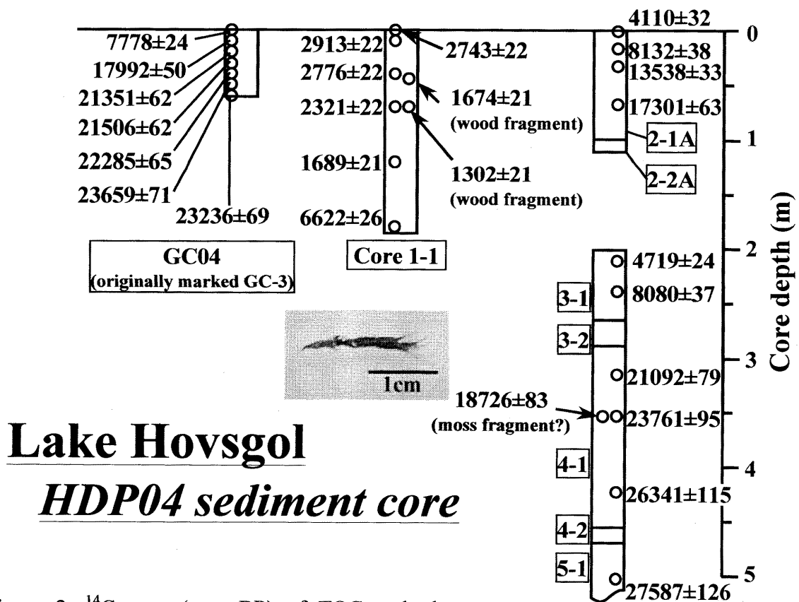
Figure 2. ^{14}\text{C} ages (year BP) of TOC and plant residue in the HDP04 sediment cores from Lake Hovsgol, Mongolia.
